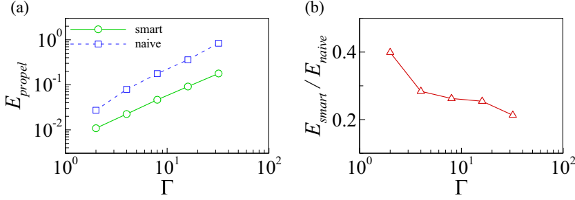
FIG. 10. (a) The propelling energy consumed by the smart agent and the naive agent, (b) the ratio of energy consumed by the smart agent to that of the naive agent as a function of \Gamma .
