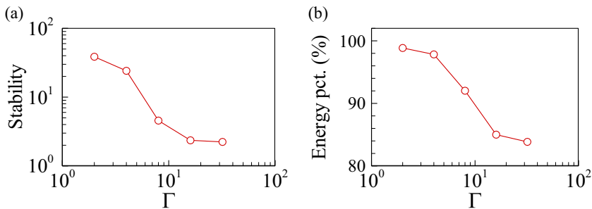
FIG. 4. (a) The stability of the first POD mode and (b) the energy contained in the first POD mode at various \Gamma .
