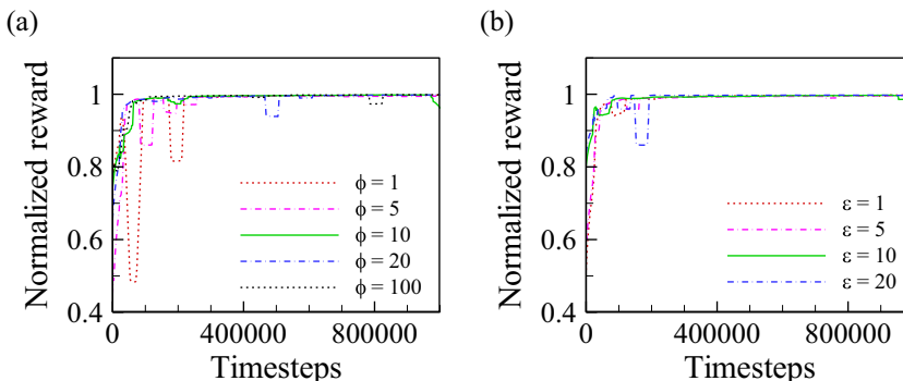
FIG. 13. Sensitivity of the hyperparameters in the reward function: (a) the penalty \phi when the agent is out of the flow domain and (b) the reward scale coefficient \epsilon .
