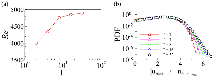
FIG. 2. (a) Reynolds number and (b) probability density functions (PDFs) of normalized velocity magnitude \|\mathbf{u}_{fluid}\| / \|\mathbf{u}_{fluid}\|_{rms} , for various \Gamma at Ra = 10^8 and Pr = 0.71 .
