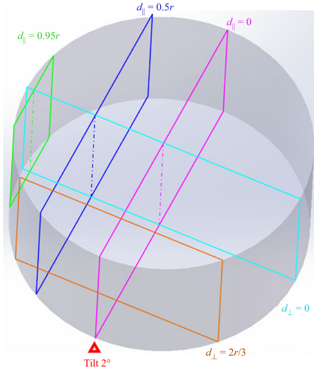
Figure 1. Sketch of the convection cell and the five planes where the planar PIV velocity measurements are conducted. The cell is tilted by 2^\circ , and d_{\parallel} = 0 is the central plane of the LSC. The planar PIV velocity measurements were conducted in the d_{\parallel} = 0 plane and two planes ( d_{\parallel} = 0.5r and d_{\parallel} = 0.95r ) in parallel to the d_{\parallel} = 0 plane, and two planes ( d_{\perp} = 0 and d_{\perp} = 2r/3 ) perpendicular to the d_{\parallel} = 0 plane.
